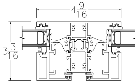
⑤ OPER/OPER T-BAR
