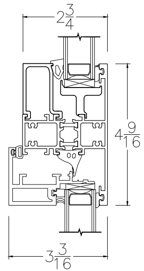
⑥ FIXED/OPERABLE TRANSOM
