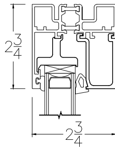
⑤ OPER/OPER T-BAR
