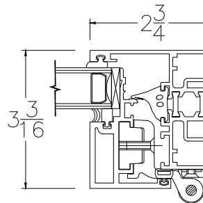
③ OPERABLE JAMB W/HINGE
