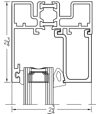
⑥ FX HEAD/JAMB
